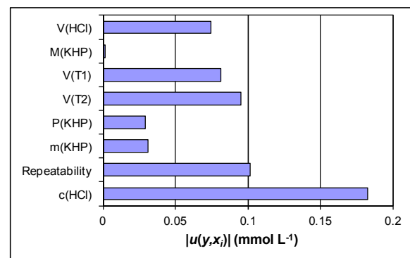
Figure A3.6: Uncertainties in acid-base titration
